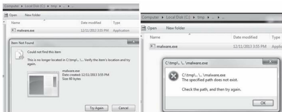
Figure 148 - Hiding Files
