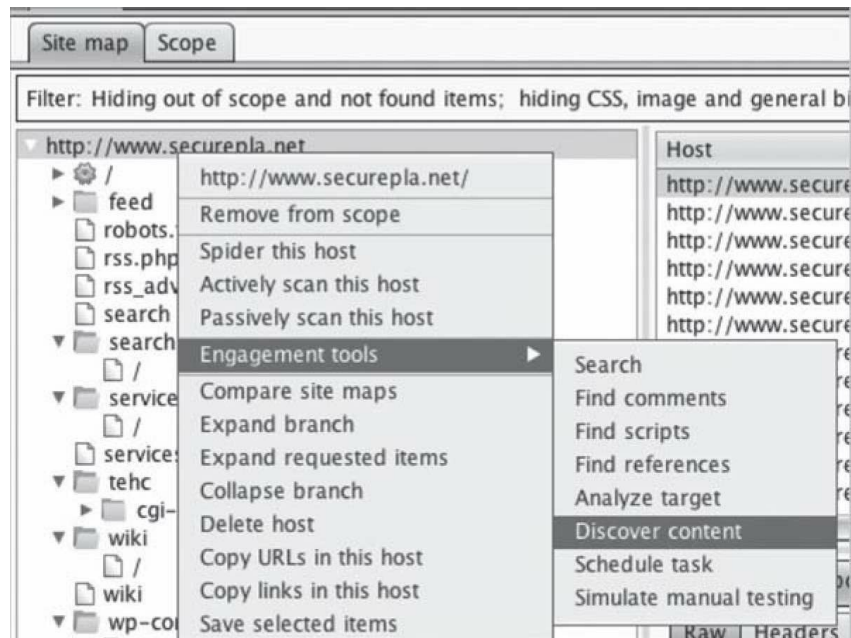
Figure 21 - Discovering Content
