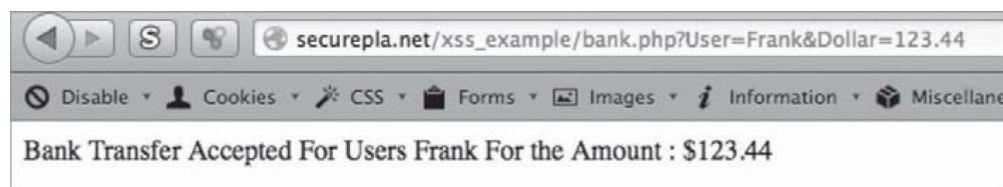
Figure 46 - CSRF Example
