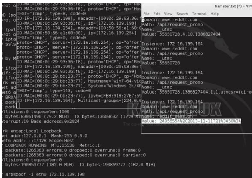
Figure 91 - Hamster Results
