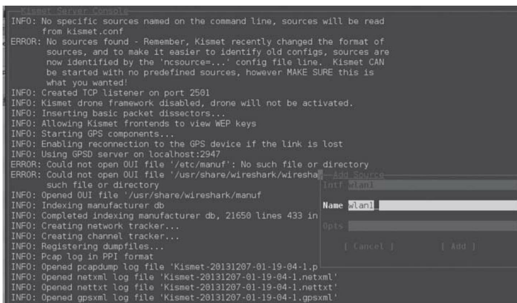
Figure 115 - Kismet Configuration
