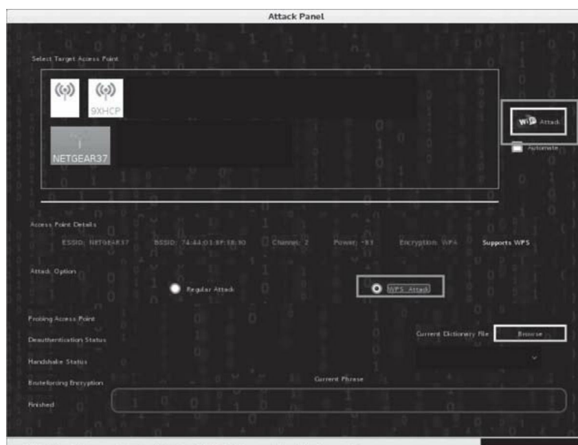
Figure 123 - WPS Attack
