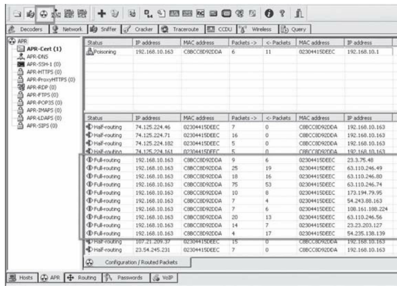
Figure 86 - Successful Poisoning
