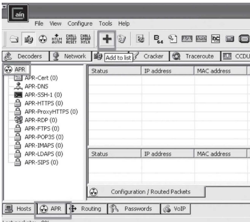
Figure 84 - APR List
