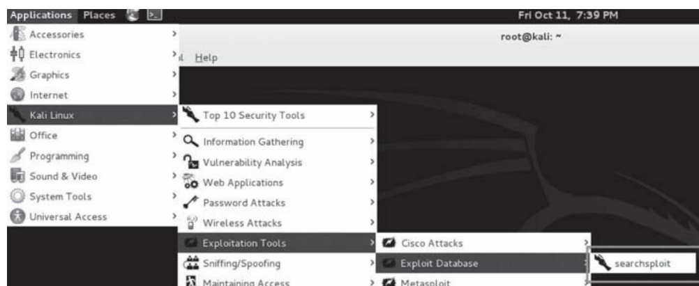
Figure 138 - Searchsploit
