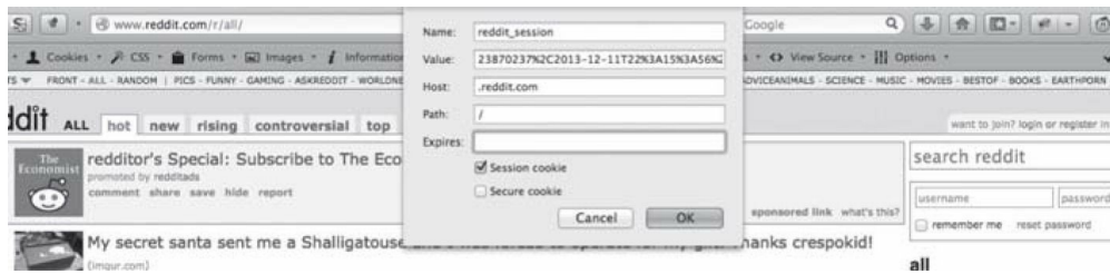
Figure 92 - Replacing Cookies
