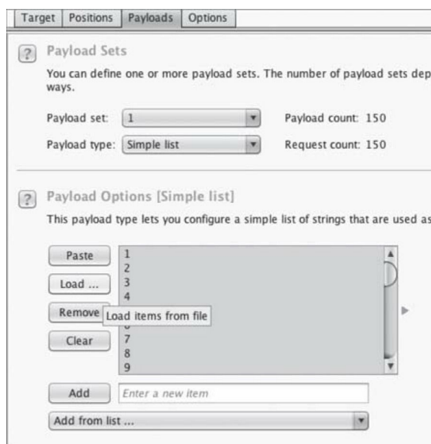
Figure 57 - Burp List
