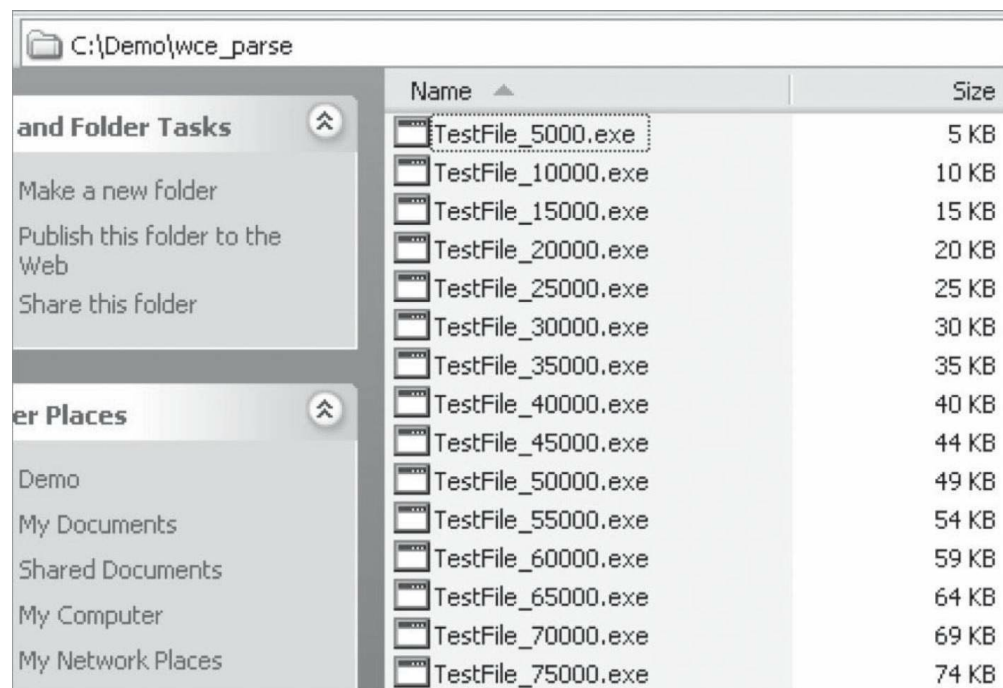
Figure 126 - Evade Output
