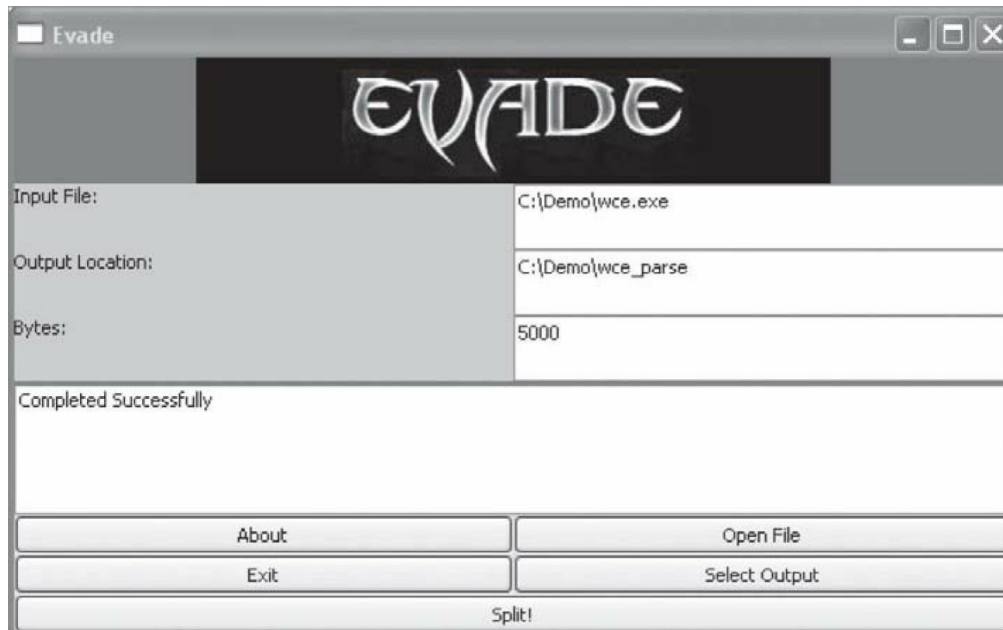
Figure 125 - Evade
