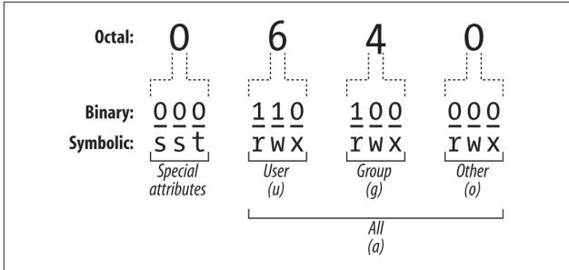
Figure 6. File permission bits explained
