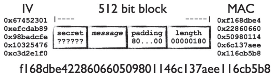
Figure 6.1 Contents of a Single Round MAC.
