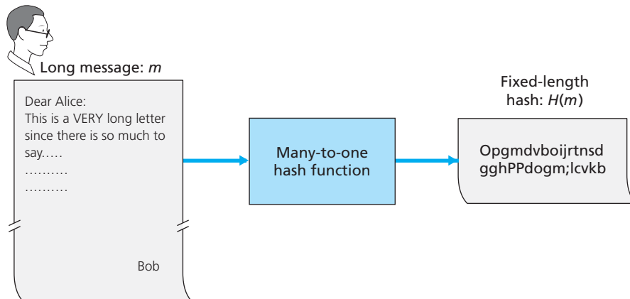
Figure 8.7 ♦ Hash functions
