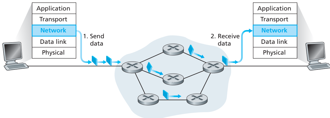
Figure 4.5 ♦ Datagram network
