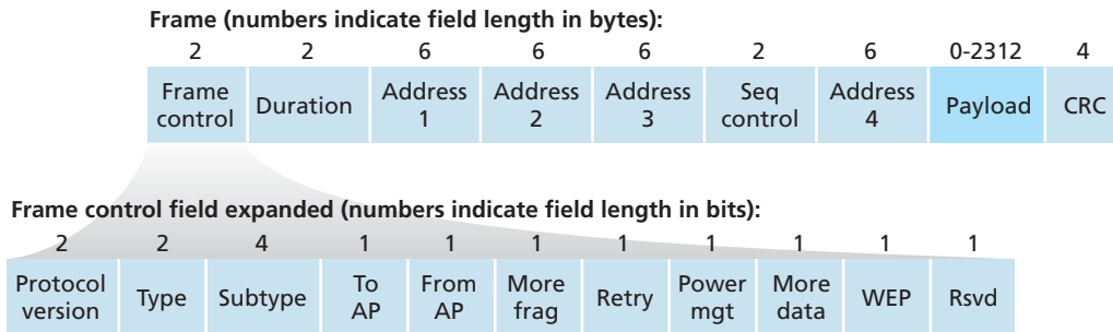
Figure 6.13 ♦ The 802.11 frame
