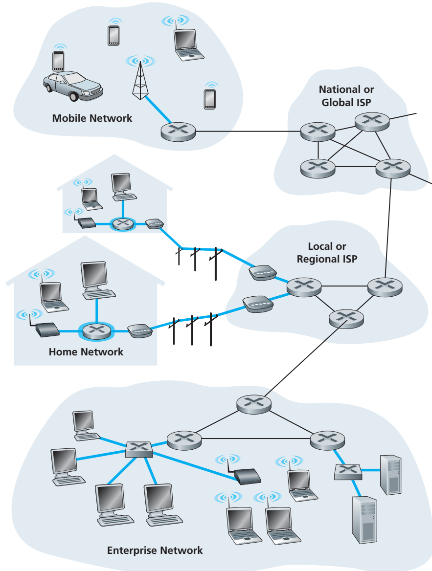
Figure 1.4 ♦ Access networks
