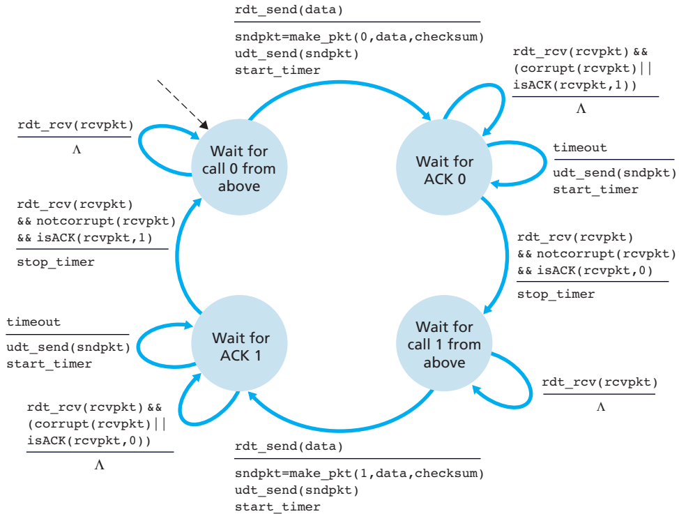
Figure 3.15 ♦ rdt3.0 sender
