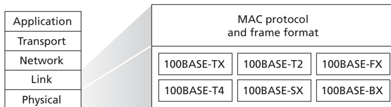
Figure 5.21 ♦ 100 Mbps Ethernet standards: a common link layer, different physical layers
