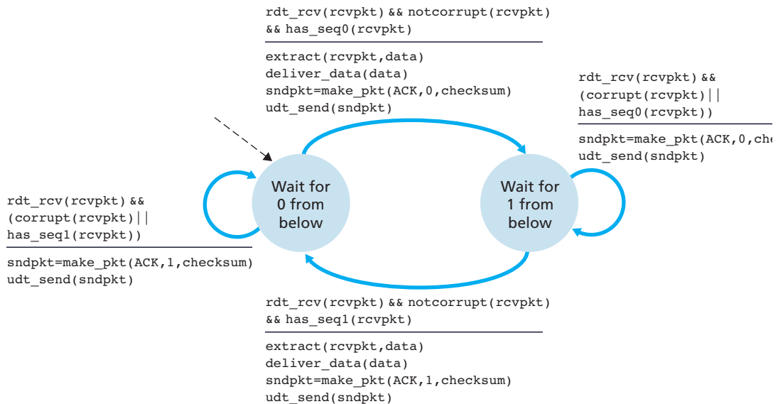
Figure 3.14 ♦ rdt2.2 receiver
