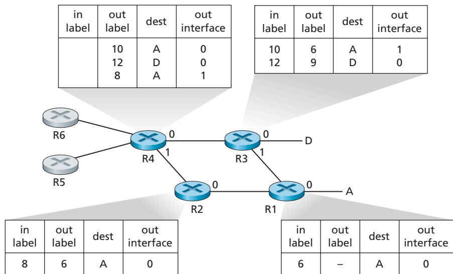
Figure 5.29 ♦ MPLS-enhanced forwarding
